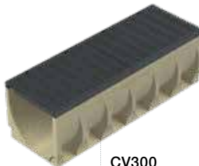
CV300 300w x 325d
